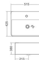
785 HALF WALL HUNG BASIN L515, W425, H380mm
