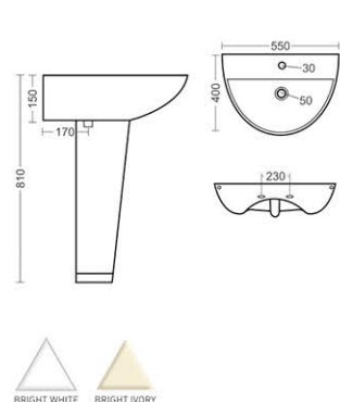
BASIN - 711 L550, W400, H495mm
