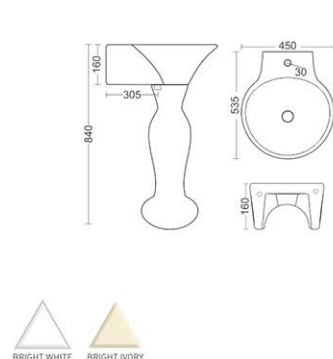
BASIN - 773 L535, W450, H160mm
