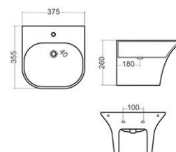
720 HALF WALL HUNG BASIN L375, W355, H260mm
