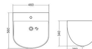
767 HALF WALL HUNG BASIN L560, W460, H340mm
