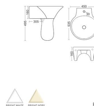
BASIN - 773 L535, W450, H160mm
