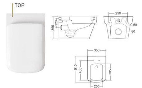
703 WALL HUNG CLOSET WASH DOWN L510, W350, H365mm
