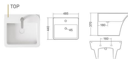
704 HALF WALL HUNG BASIN L485, W440, H370mm
